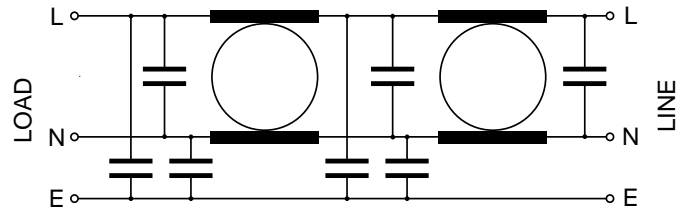
Circuit Schematic
