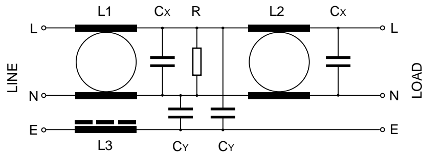
Circuit Schematic
